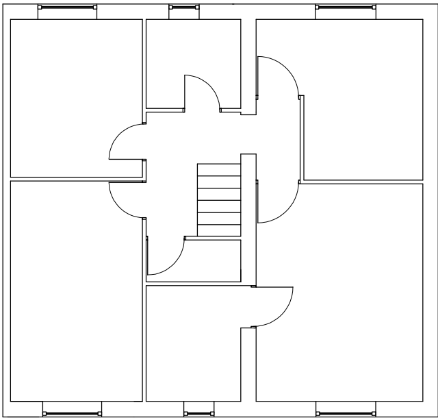
EXISTING FIRST FLOOR 1:100
