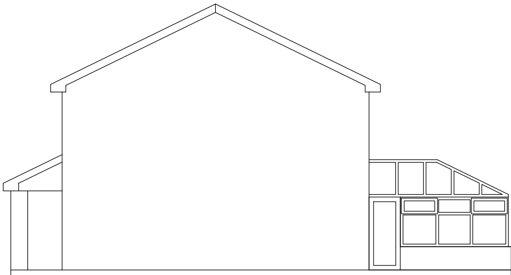
EXISTING GABLE END ELEVATION 1:100
