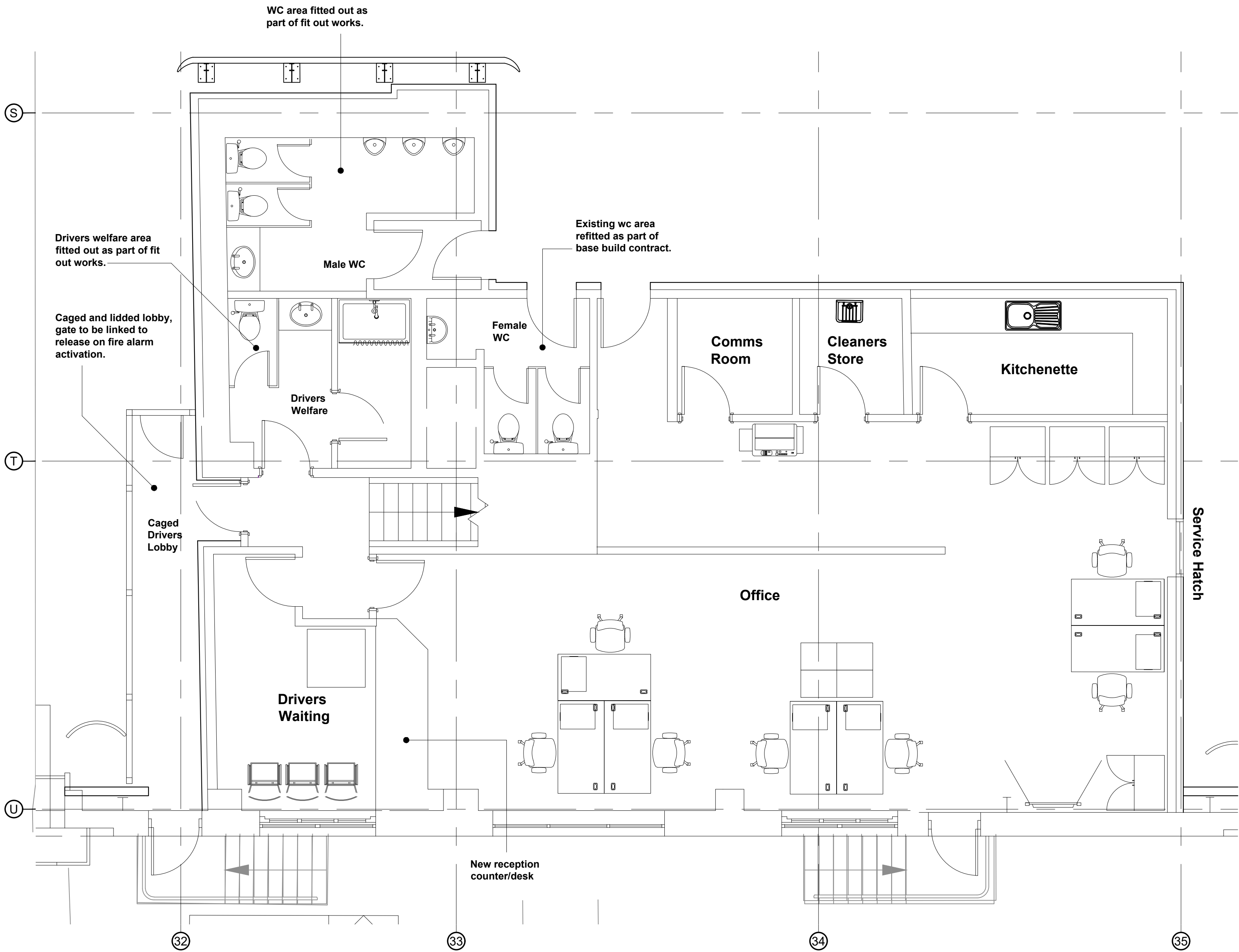
Proposed Pod Office - Ground Floor Scale 1:50
