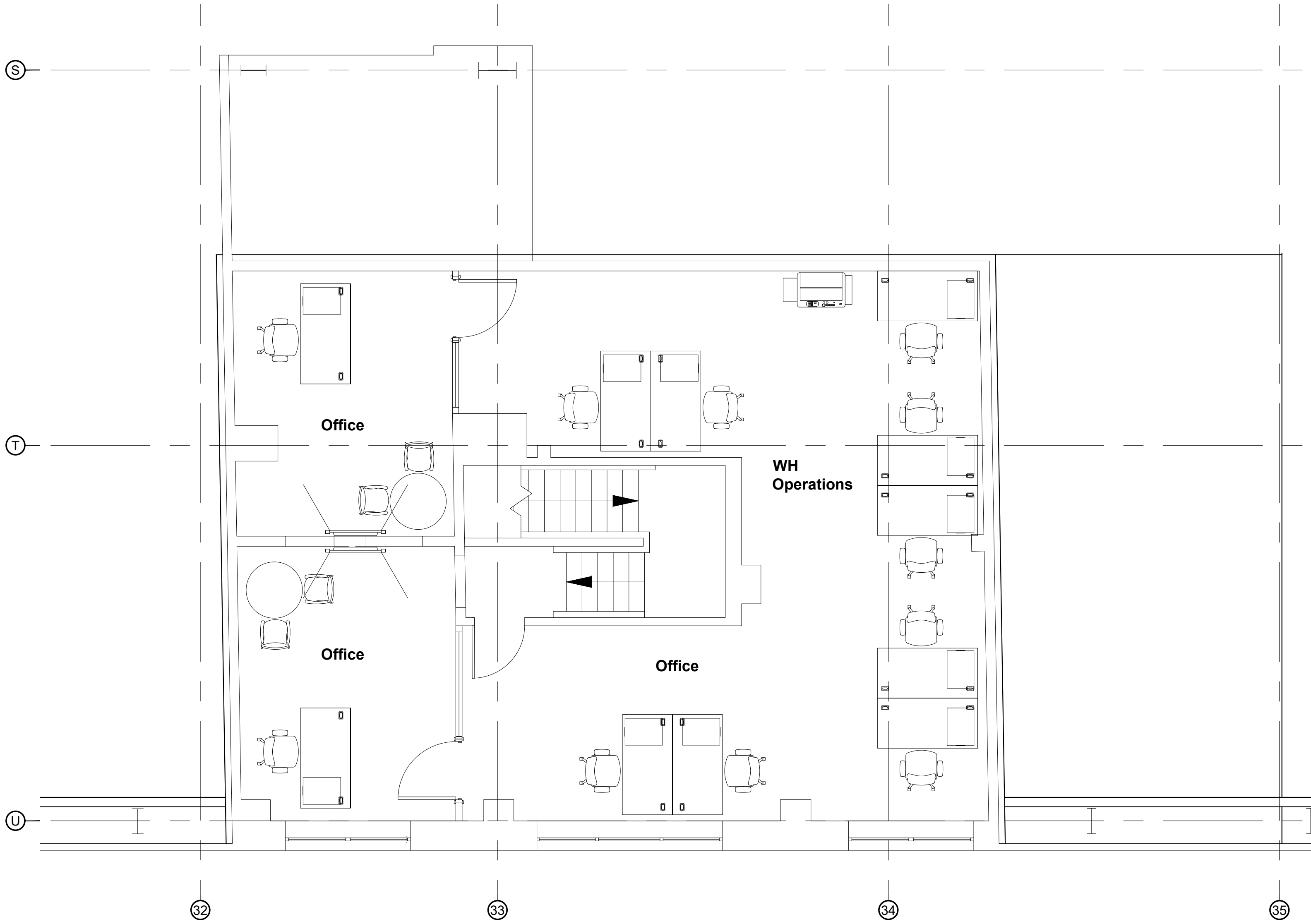
Proposed Pod Office - First Floor Scale 1:50
