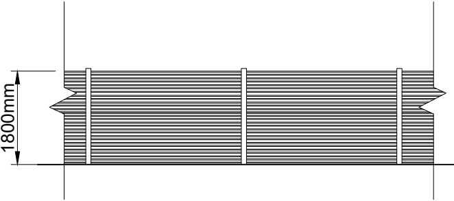
TIMBER FENCE DETAIL (PROPOSED) Scale 1:100
