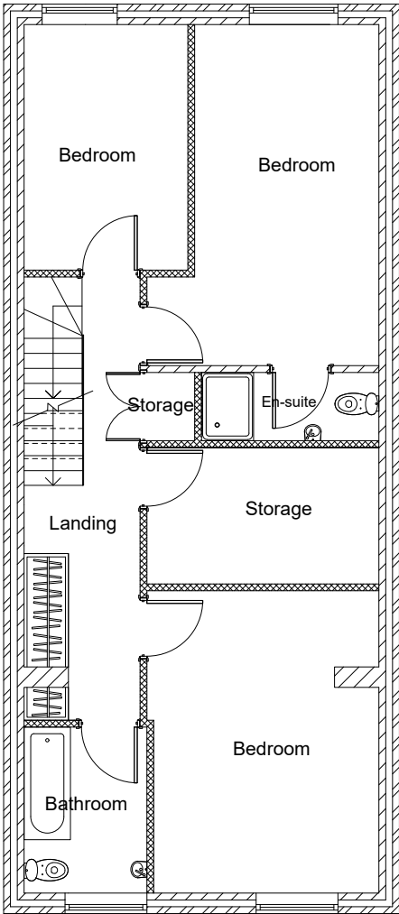
FIRST FLOOR PLAN (PROPOSED)
