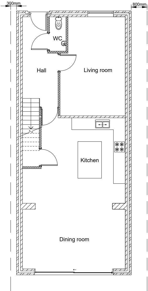
GROUND FLOOR PLAN (PROPOSED)
