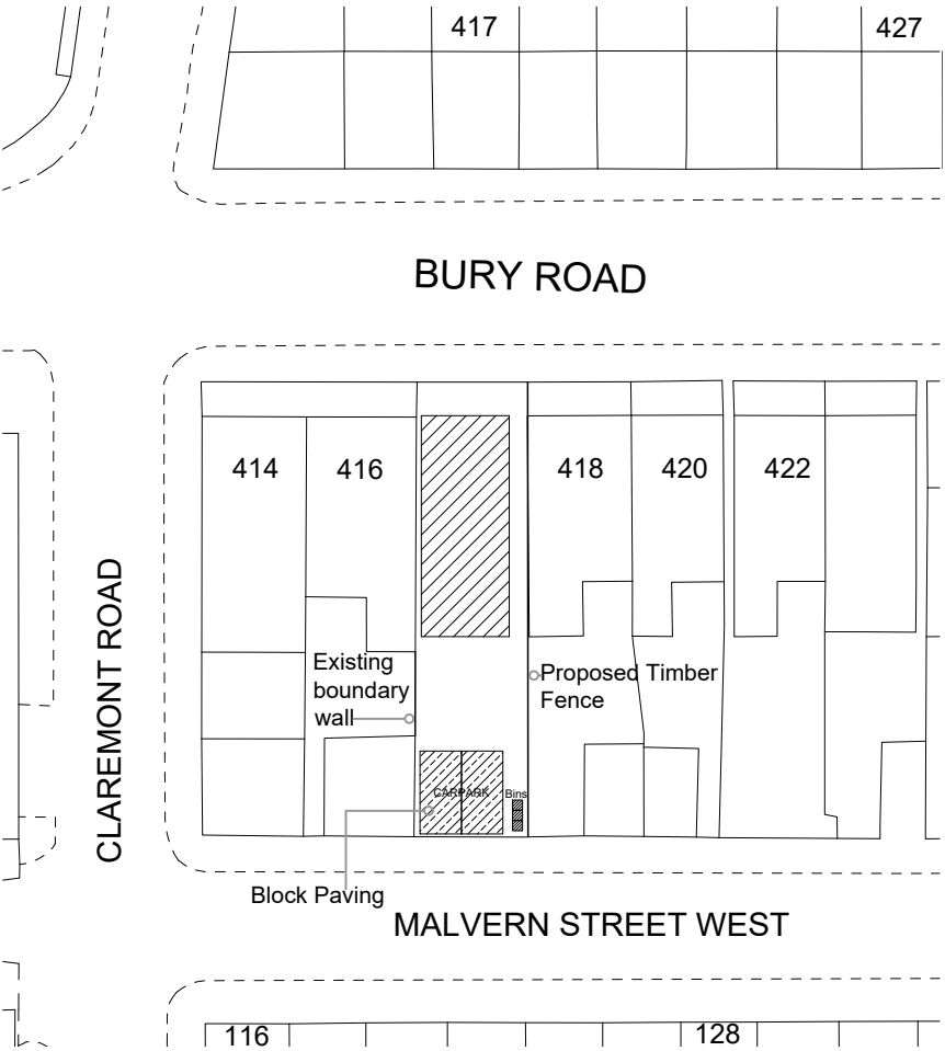
SITE PLAN (PROPOSED)
