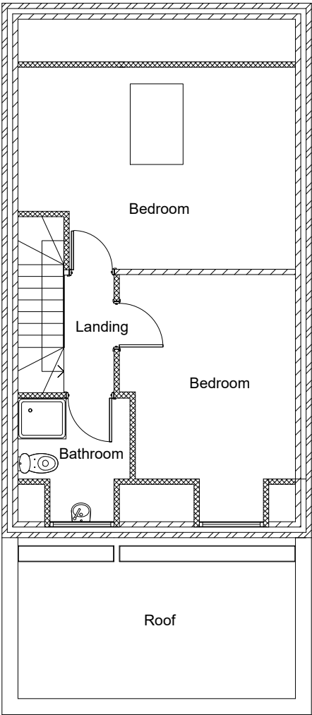
SECOND FLOOR PLAN (PROPOSED)
