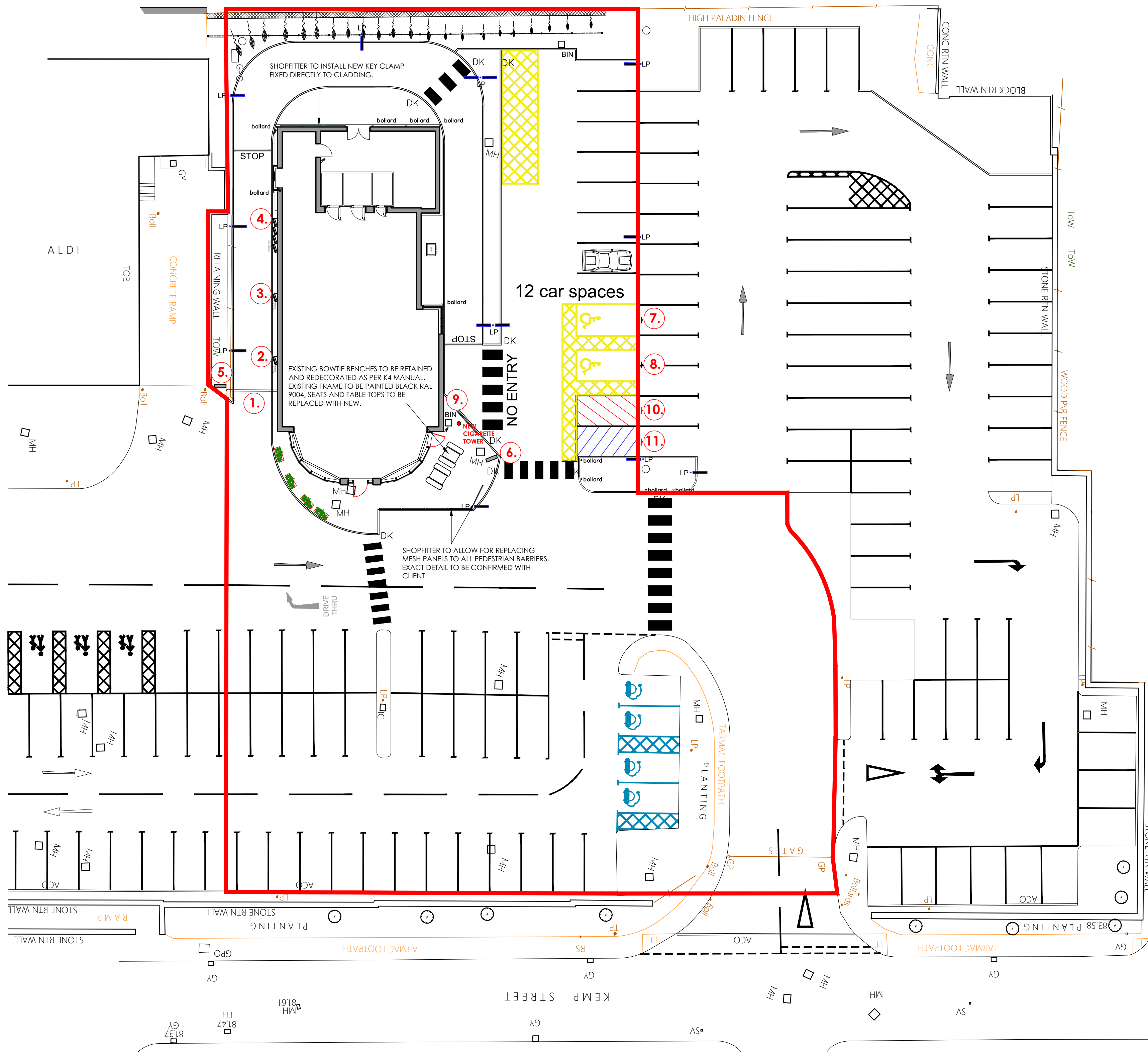
proposed site signage plan scale - 1:50 @ A1 / 1:100 @ A3
