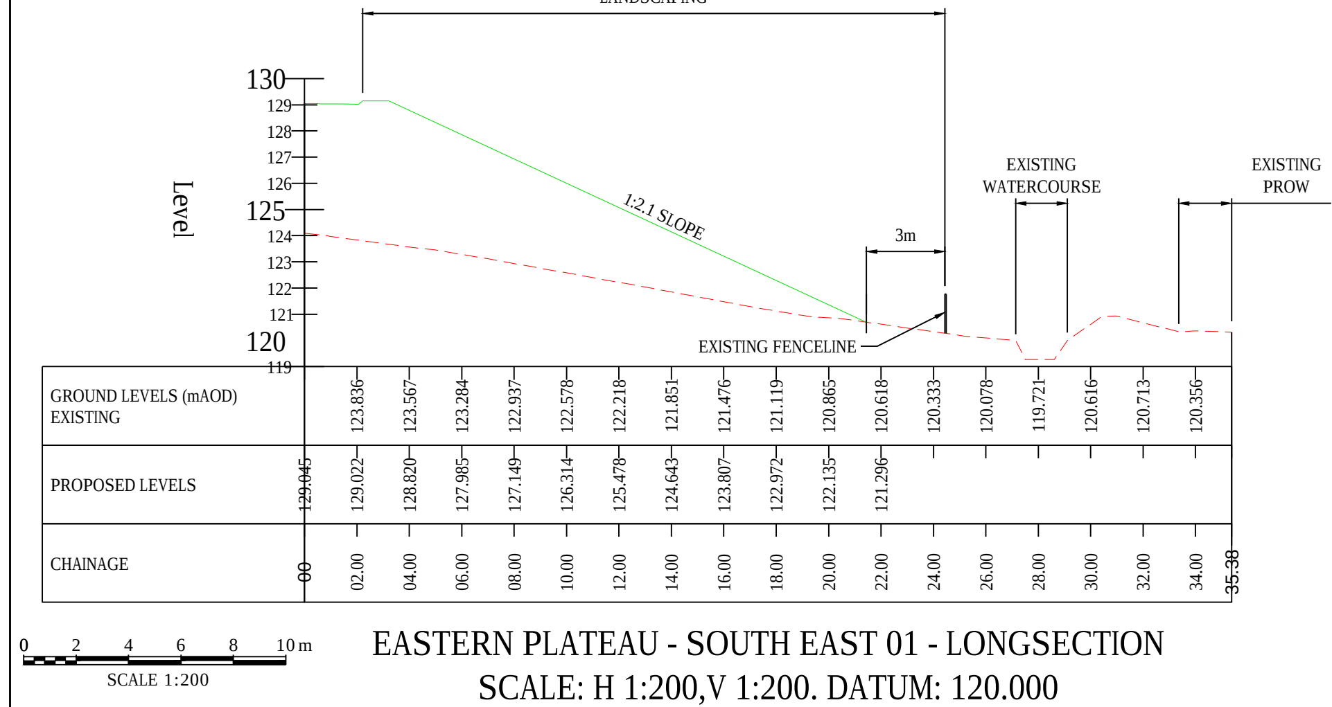
KEY + 125.235 + 130.50m EXISTING GROUND LEVELS PROPOSED GROUND LEVELS
