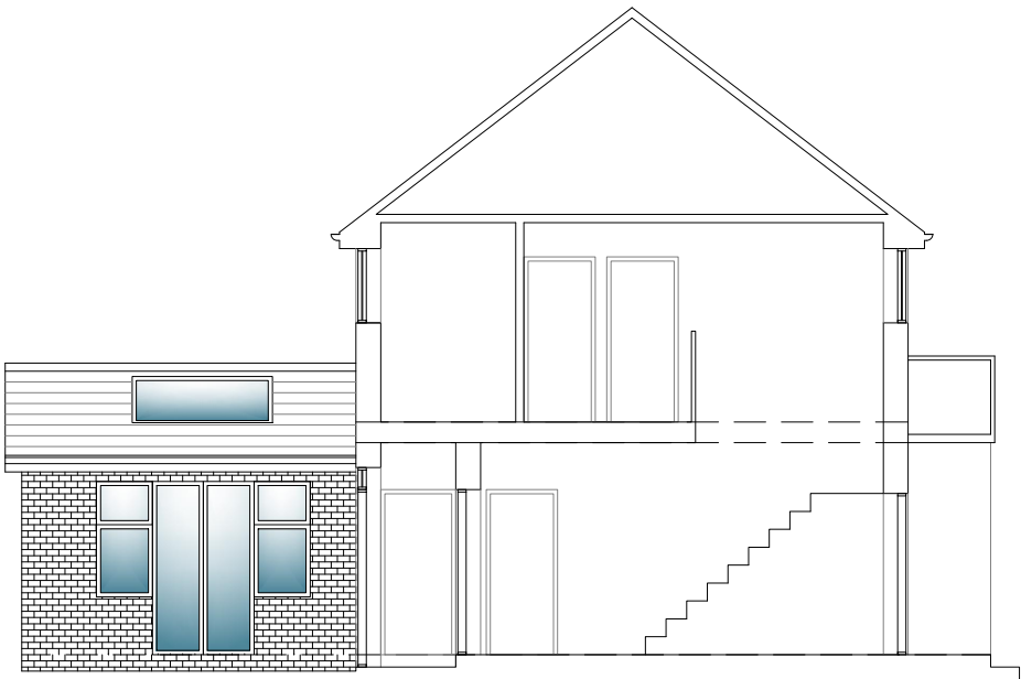
PROPOSED SECTION
