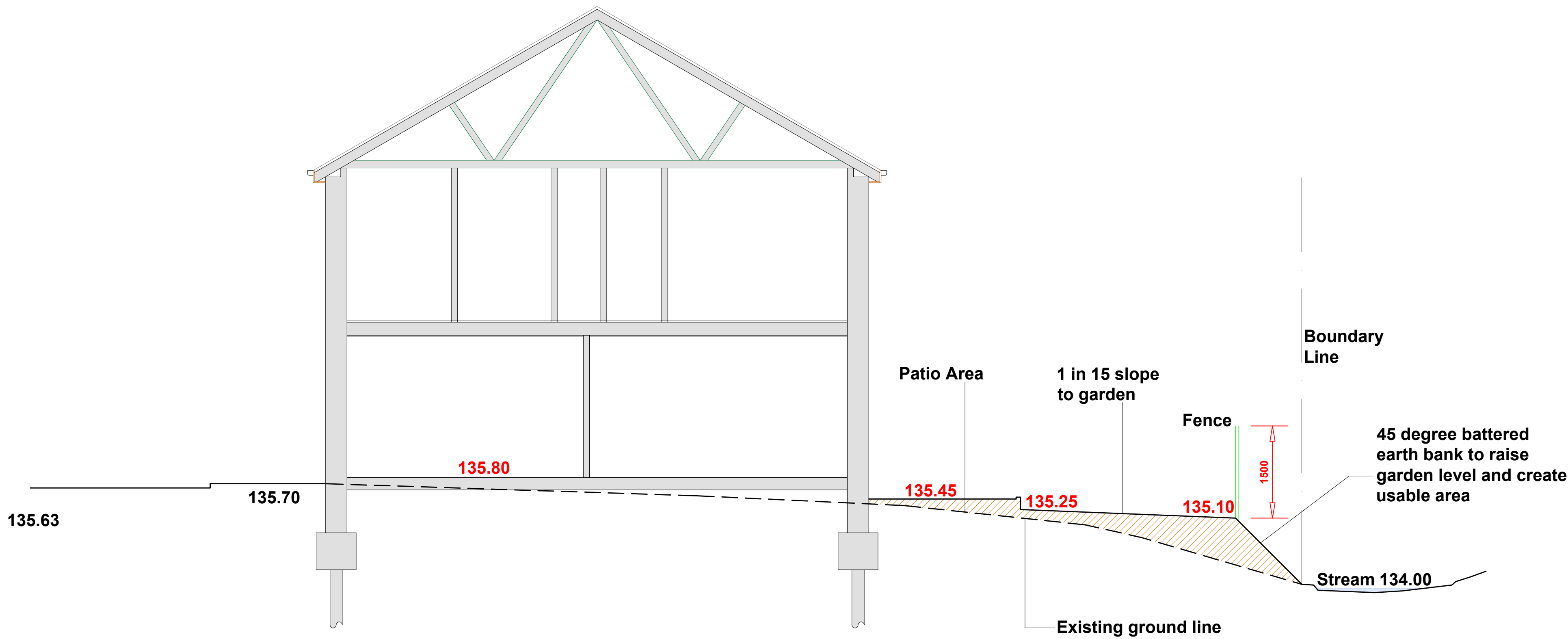
PROPOSED SITE SECTION X - X
