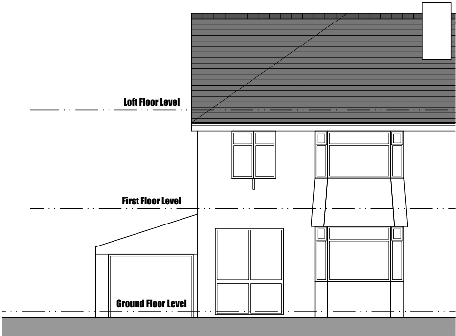
North Facing Front Elevation
