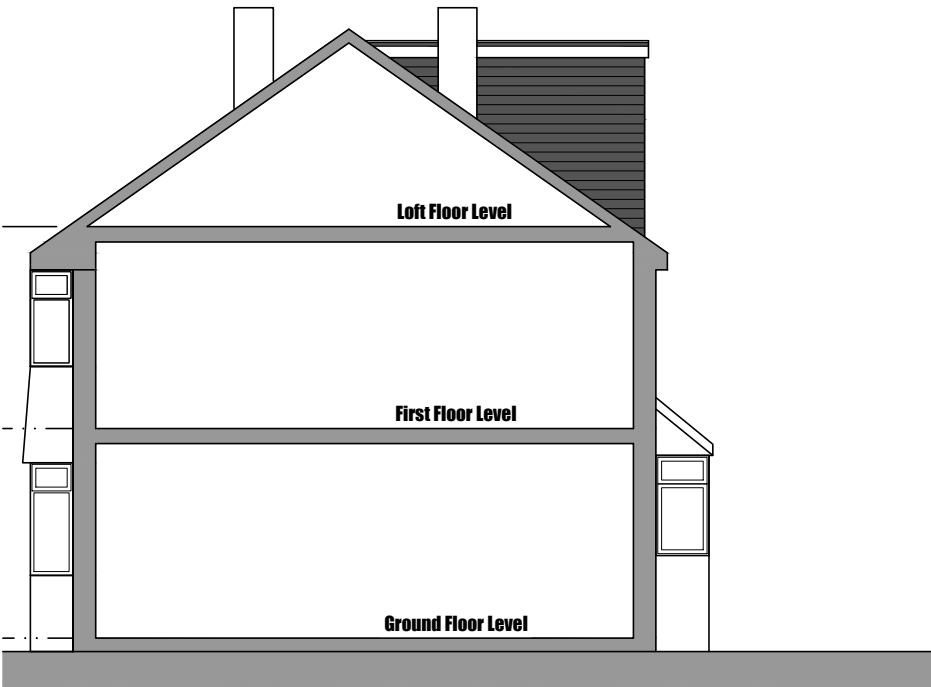
West Facing Side Elevational Section
