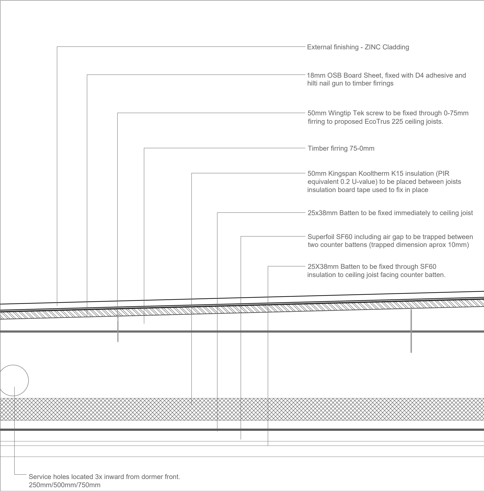
ECOTRUS CEILING JOIST DETAIL (225mm) @ 1:5
