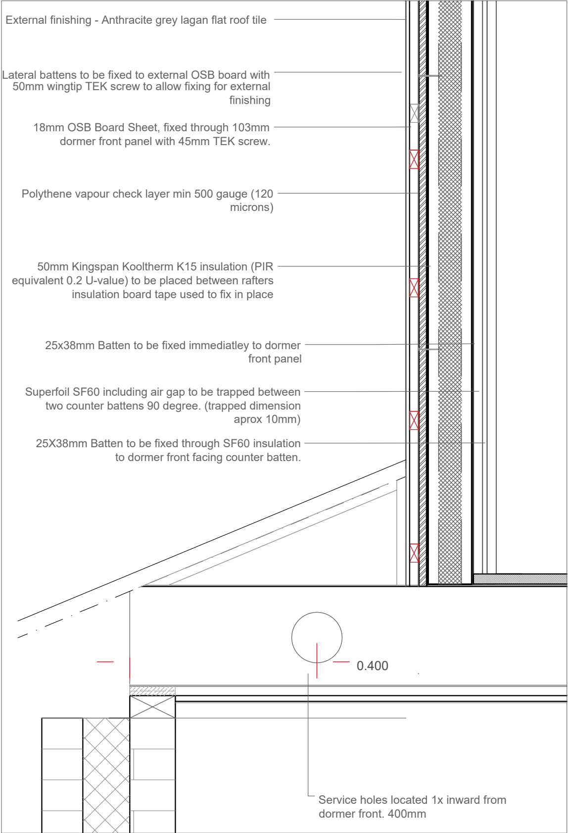
ECOTRUS DORMER FRONT CROSS SECTION (103mm DORMER FRONT PANEL & 225mm FLOOR JOIST) @ 1:5
