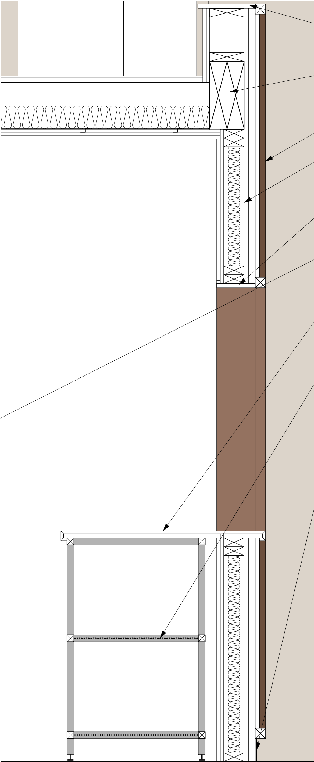
SECTION | 1:10
