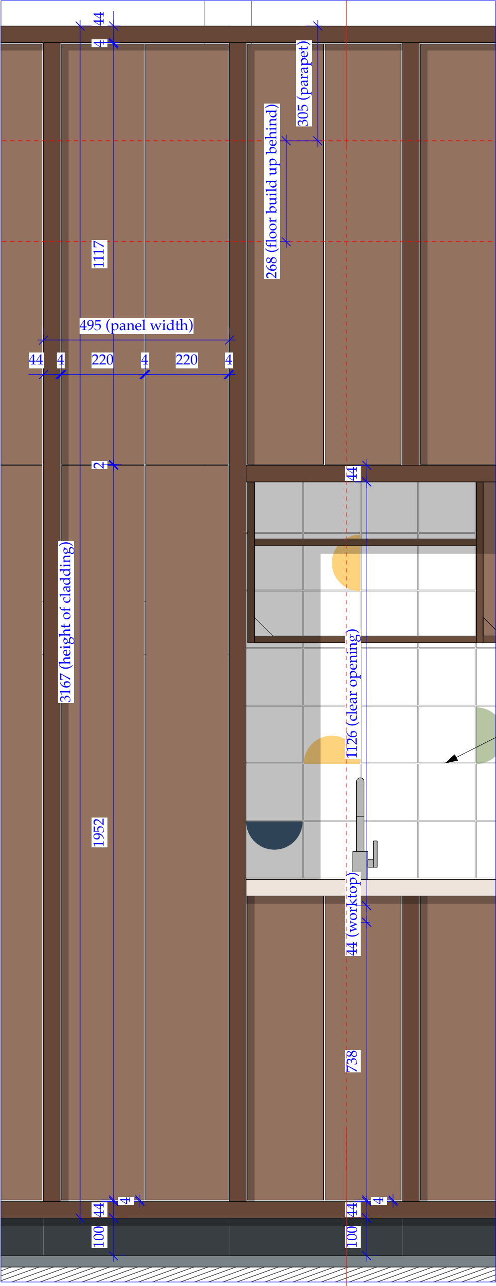
ELEVATION | 1:10
