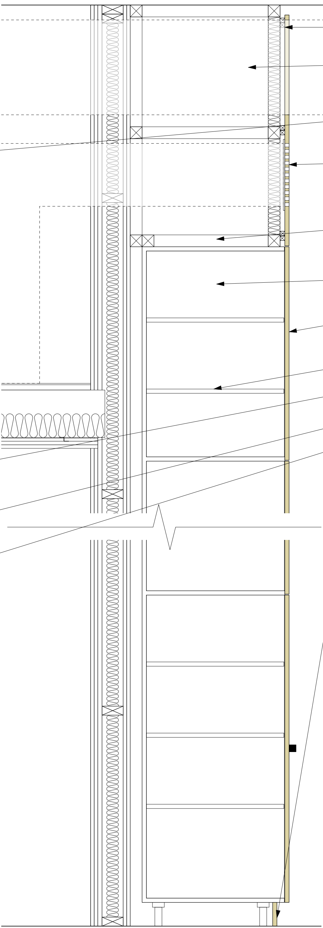
SECTION | 1:10
