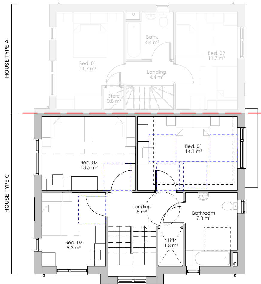
01 First Floor
