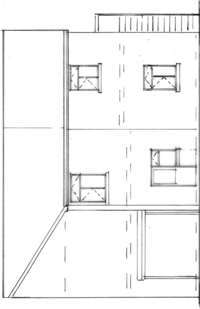
REAR ELEVATION (PROPOSED)
