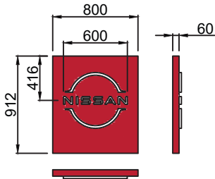
Sign G: NEXT Entry Element Size 2 Logo Illumination: Internally Illuminated with White LEDs Material: Internal Aluminium Frame 4mm ACM - Nissan Red NVR-01, RAL3001, PMS200 Scale 1:50 @ A3
