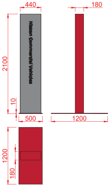
Sign E: 1x External Totem Sign (LCV) Material: Steel Base - RAL3001 Red Aluminium - RAL3001 Red Aluminium - RAL9016 White Vinyl graphic Qty: 1
