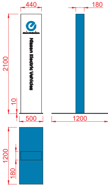
Sign F: 1x External Totem Sign (EV) Material: Steel Base - RAL5015 Blue Aluminium - RAL5015 Blue Aluminium - RAL9016 White Vinyl graphic Qty: 1
