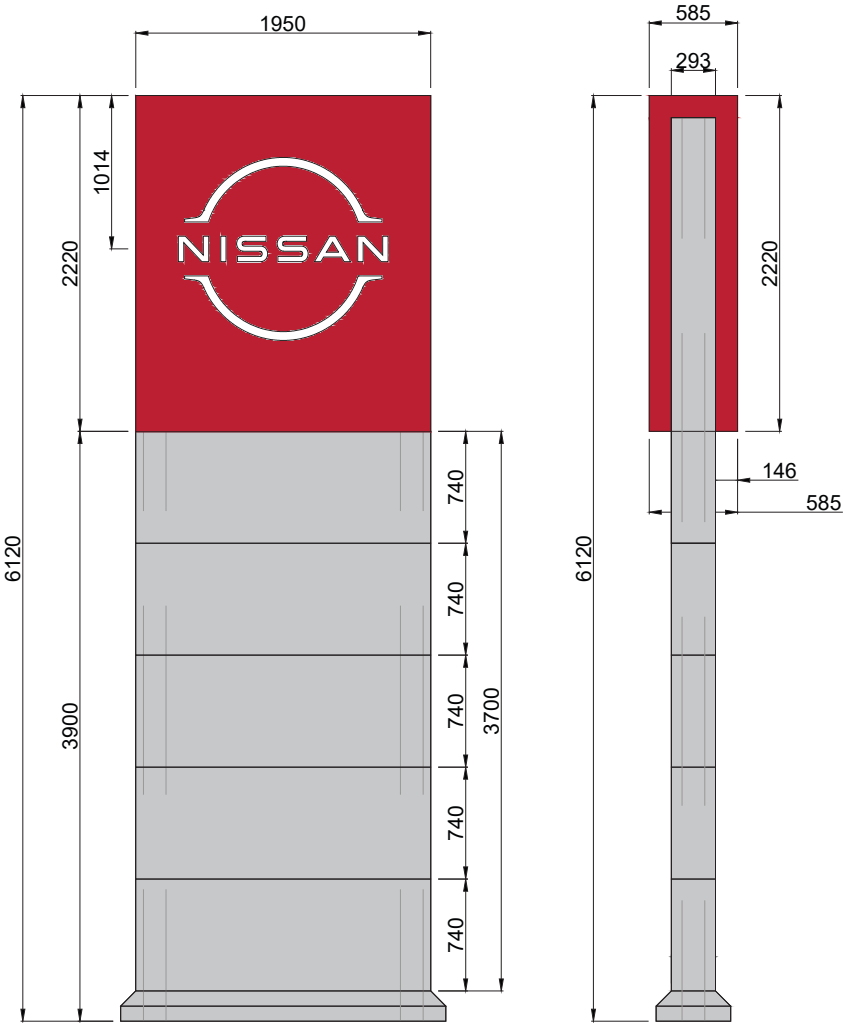
Sign H: Pylon Size 3 Logo Illumination: Internally Illuminated with White LEDs Material: Internal Steel Frame 4mm ACM - Nissan Red NVR-01, RAL3001, PMS200 4mm ACM - Silver - RAL9006, PMS Cool Grey 4 Scale 1:50 @ A3
