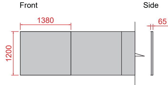
Sign A1, A2: ACM-1 Back Panels Size 4 - Ref. 4.54 Fascia length: Material: Silver ACM Silver RAL9006, PMS Cool Grey 4 Scale 1:50 @ A3
