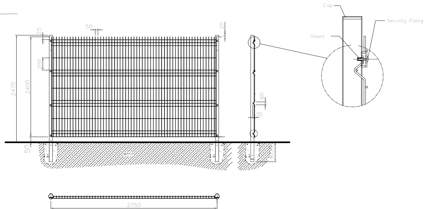
2 Detail Weldmesh Fence NTS
