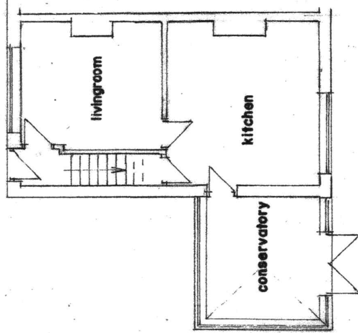
G.F. PLAN (EXISTING)
