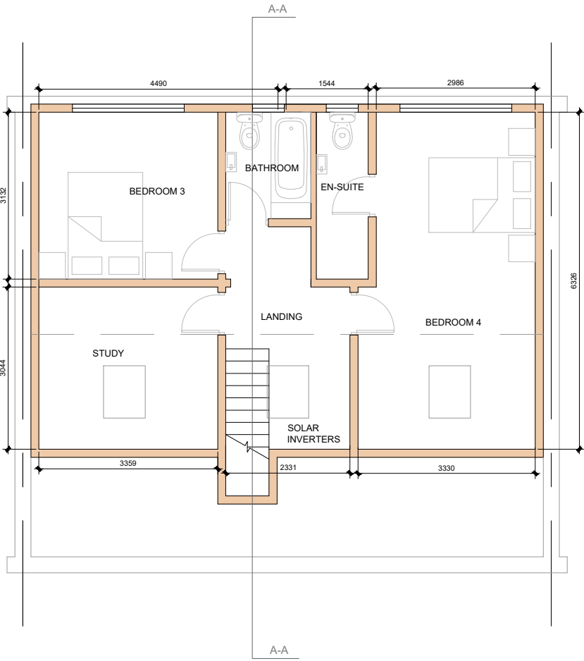
Loft floor
