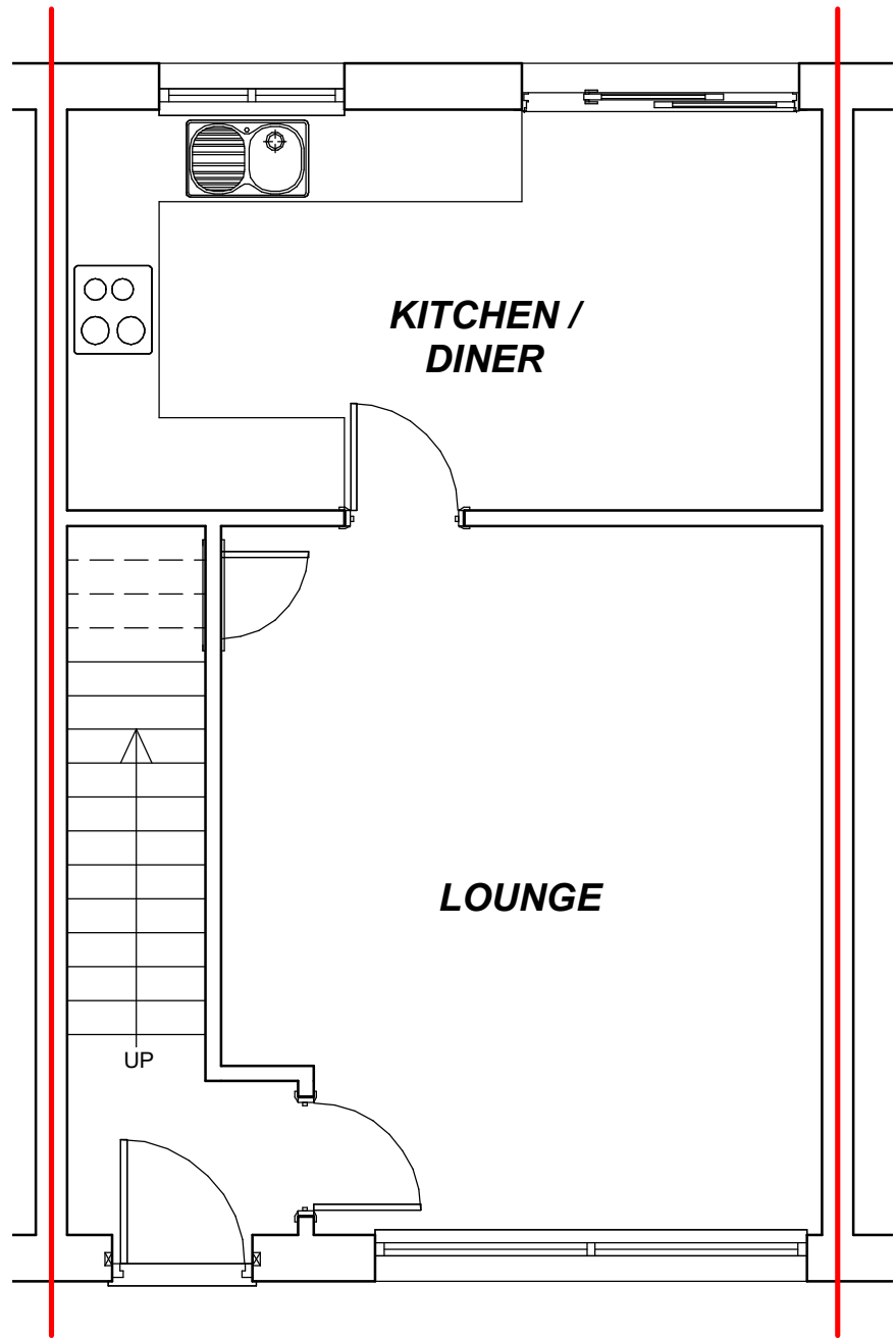
Existing Ground Floor Layout 1 : 50
