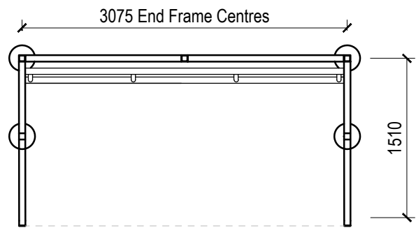
Smoking Shelter Plan Scale @ 1:50
