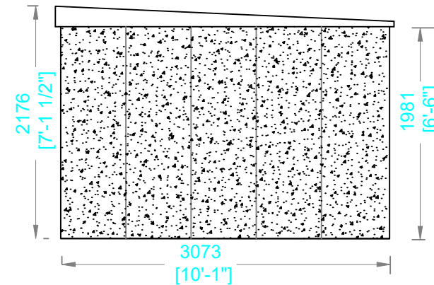
RH ELEVATION
