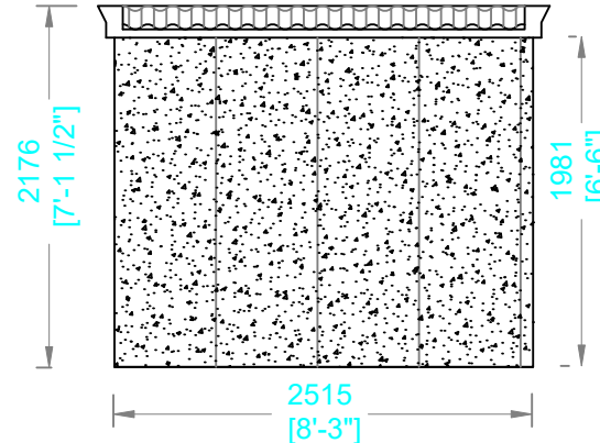
REAR ELEVATION
