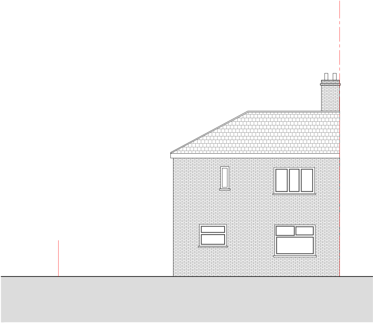
EXISTING REAR ELEVATION 1:100 @ A3
