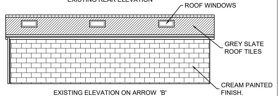
EXISTING ELEVATION ON ARROW 'B'
