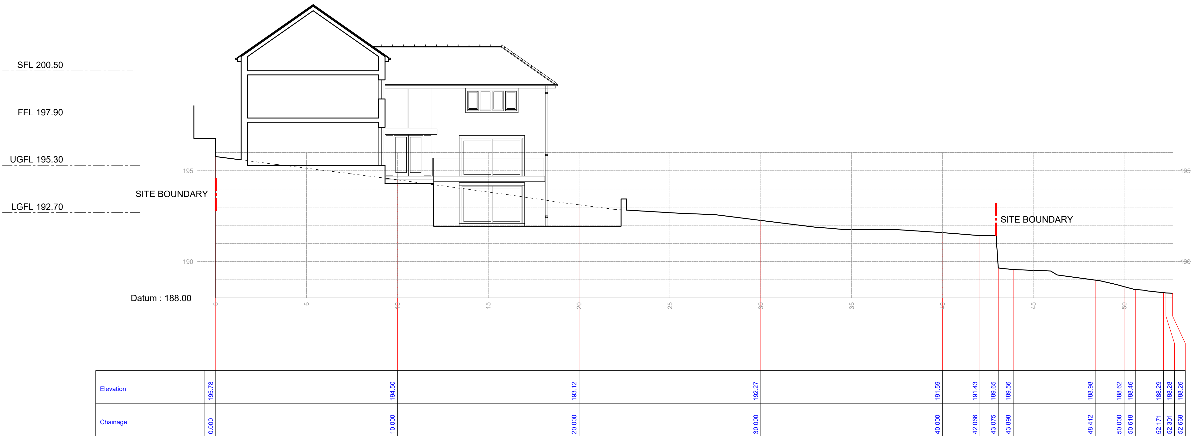
PROPOSED CROSS SECTION
