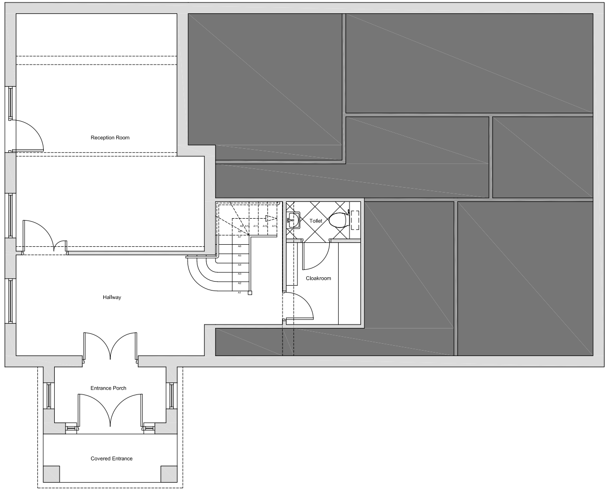
Proposed GF Plan 1:100
