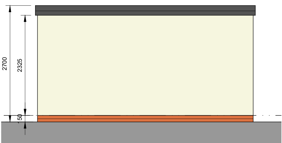
Rear Elevation
