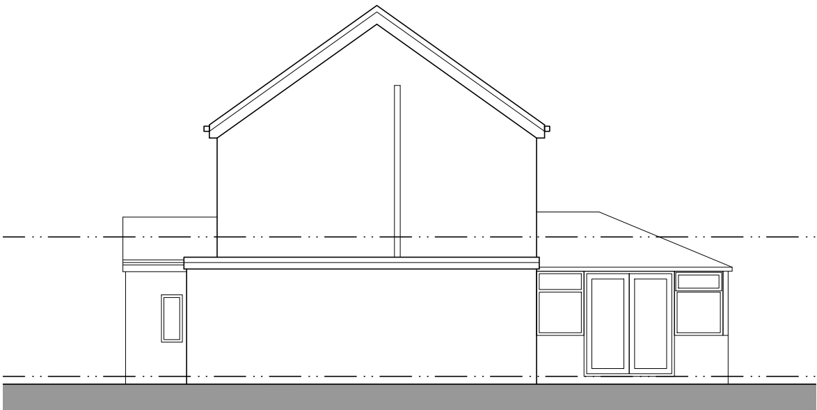
East Facing Side Elevation
