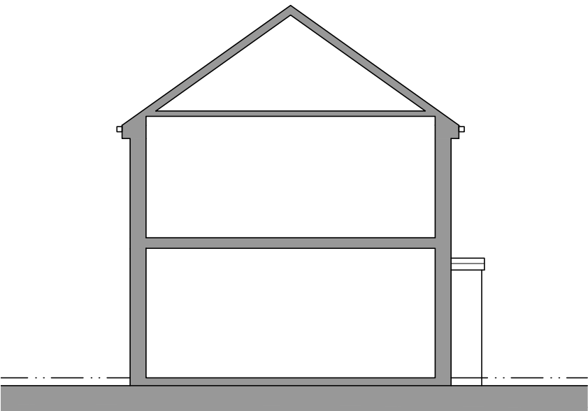
West Facing Side Elevation/Section
