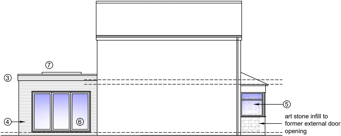
Side Elevation proposed scale 1-100
