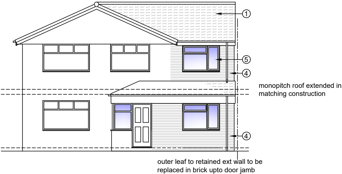
Front Elevation proposed scale 1-100
