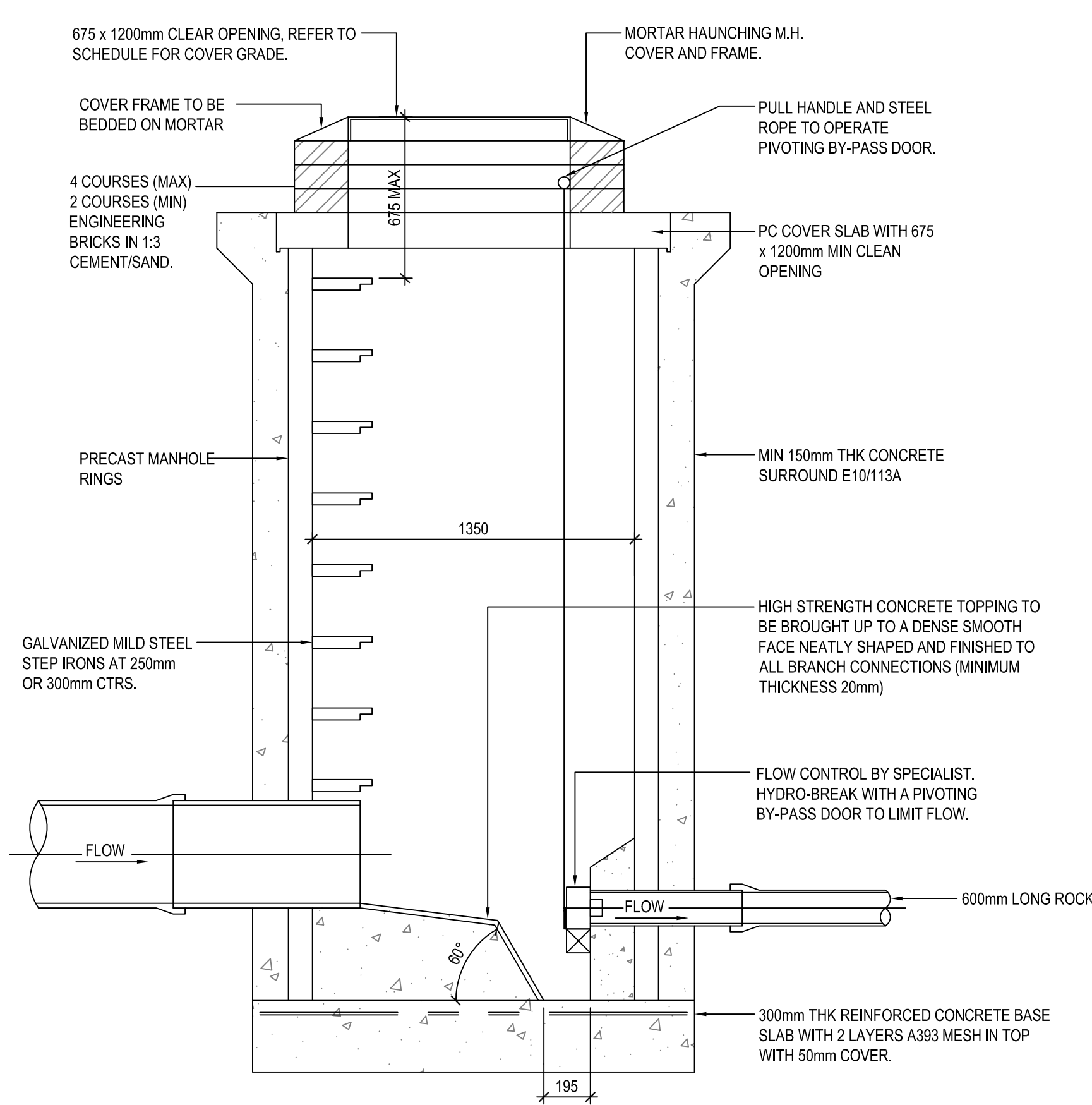
NEW HYDRO-BRAKE CHAMBER [SCALE 1:20]
