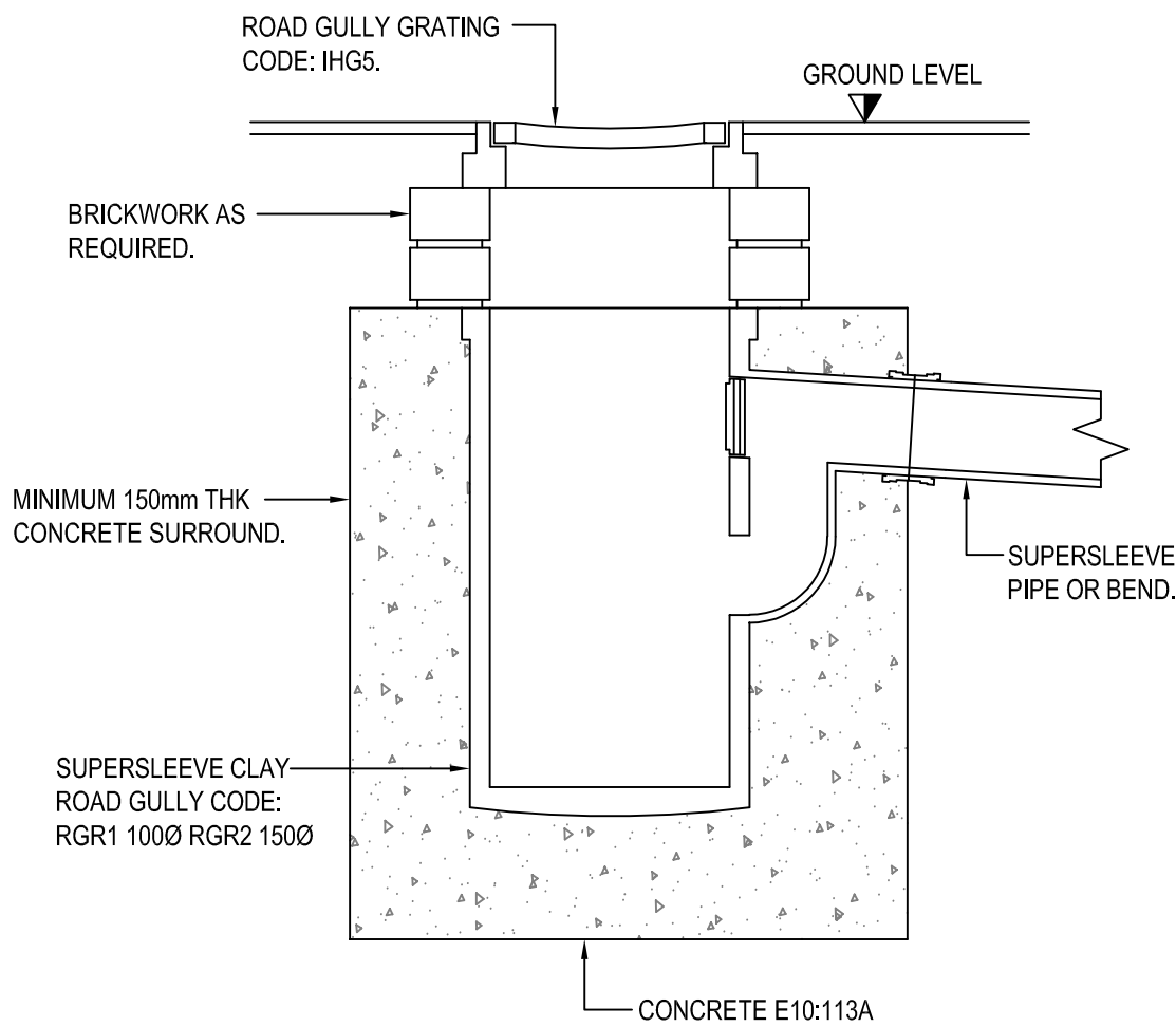
ROAD GULLY (3000 x 600Dp) [SCALE 1:10]
