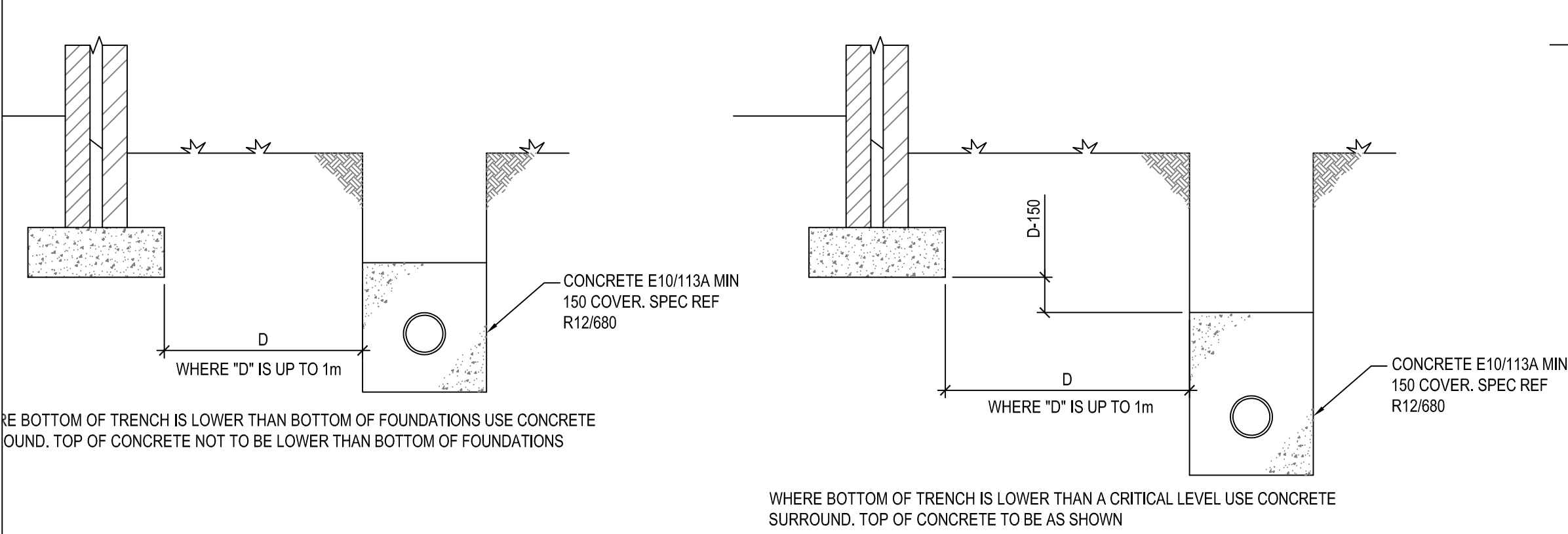
PIPES NEAR FOUNDATIONS [SCALE 1:20]
