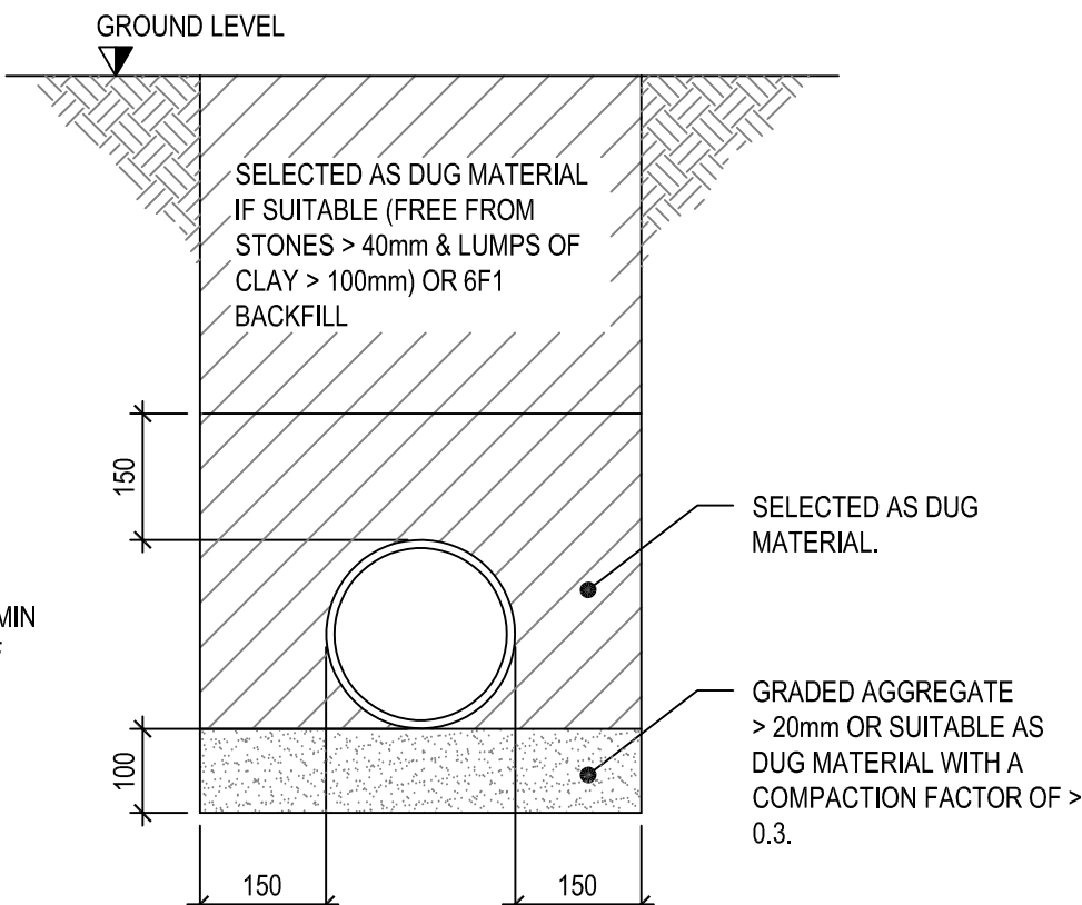
DRAIN TRENCH NOT SUBJECTED TO TRAFFIC (BEDDING CLASS N) [SCALE 1:10]
