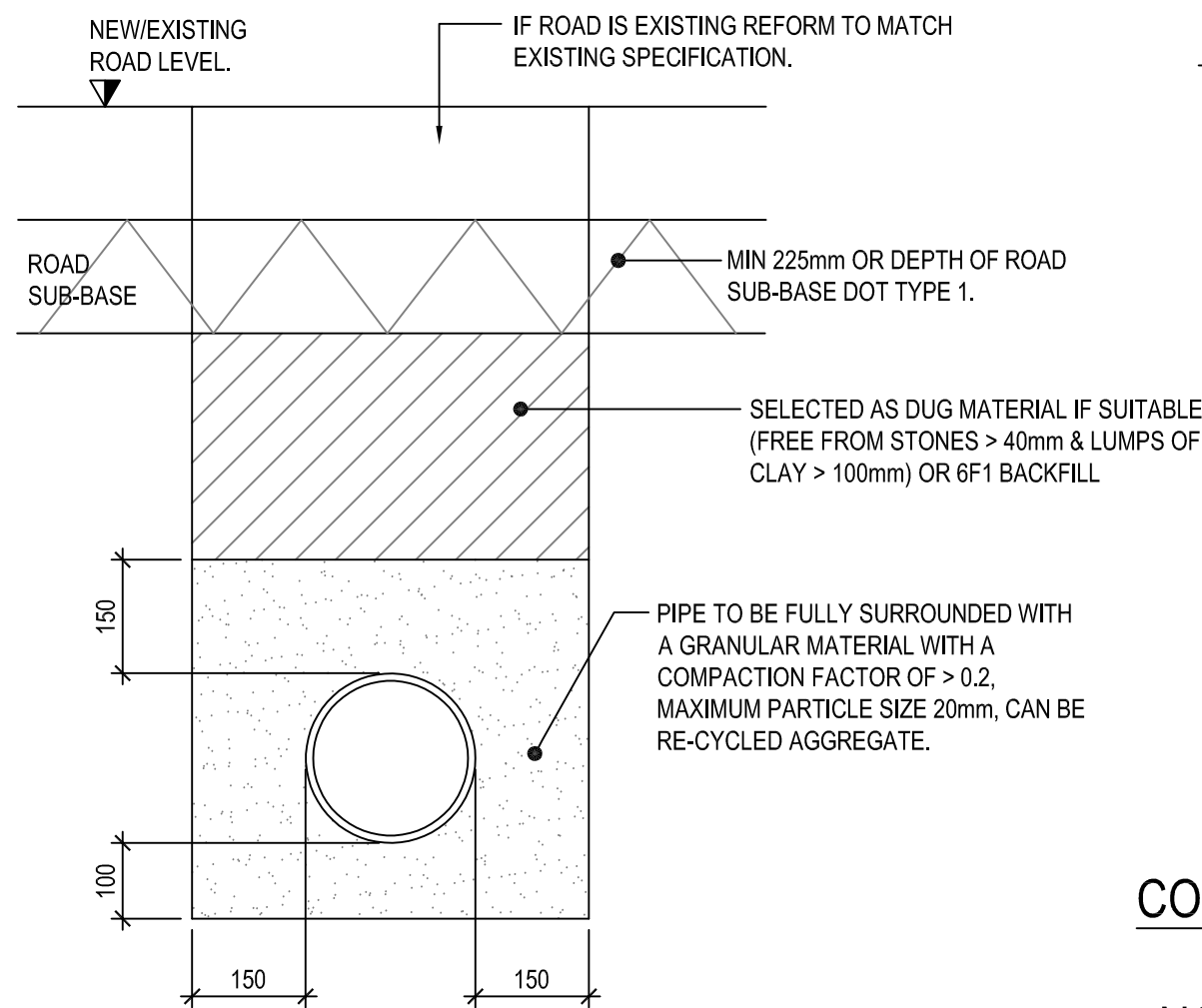
DRAIN TRENCH SUBJECTED TO TRAFFIC (BEDDING CLASS S) [SCALE 1:10 @ A1]
