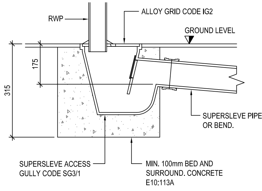
RWP DETAIL [SCALE 1:10]
