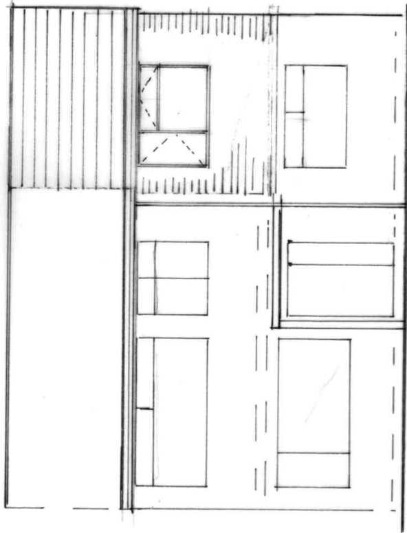
FRONT ELEVATION (PROPOSED)
