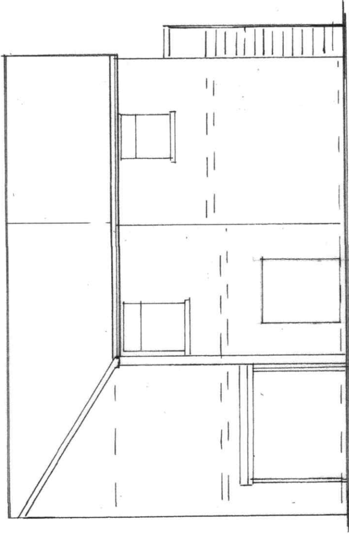
REAR ELEVATION (EXISTING)
