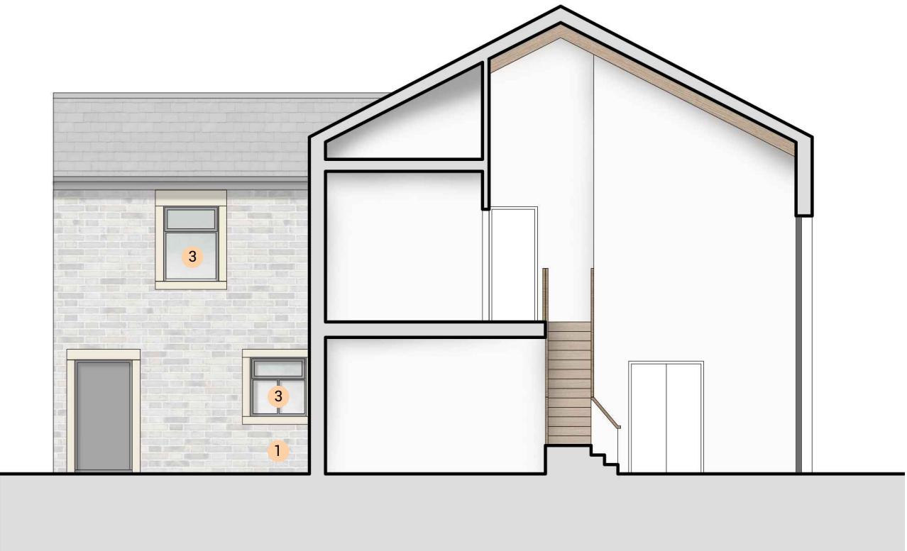
PROPOSED BARN SECTION 1:100 @ A1
