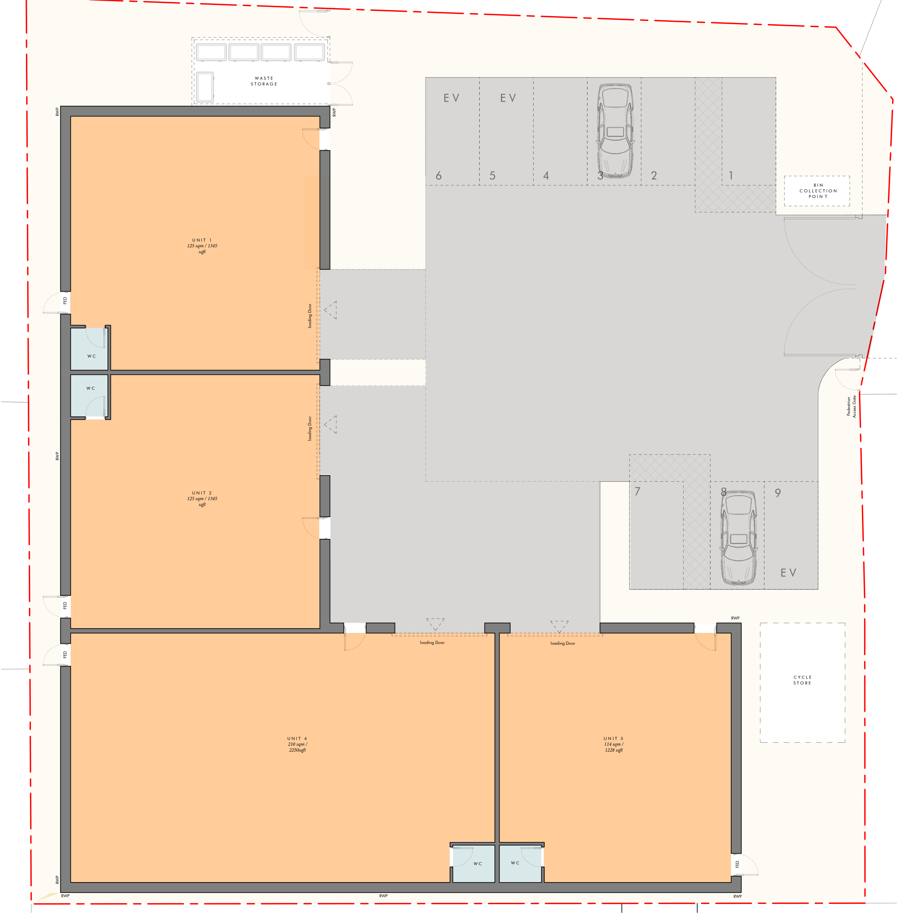
PROPOSED GROUND FLOOR PLAN 1:200 @ A2
