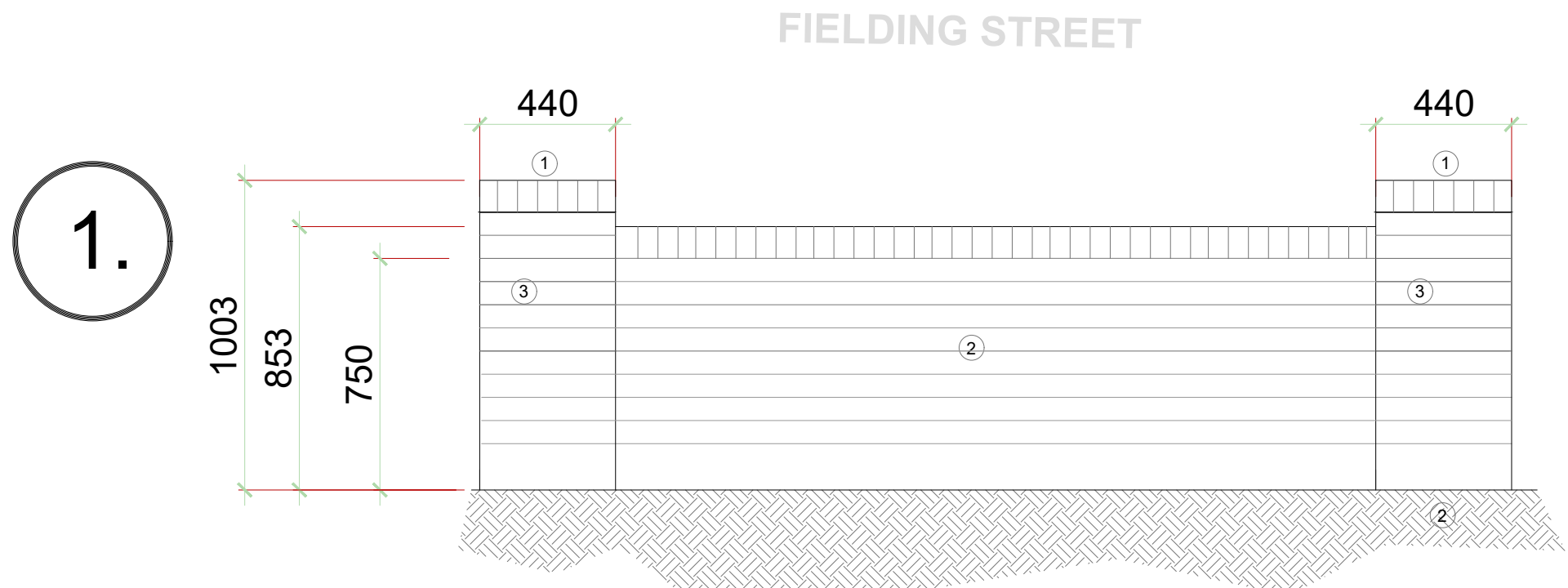
Feature wall detail 1003mm high Scale 1:20 @ A1
