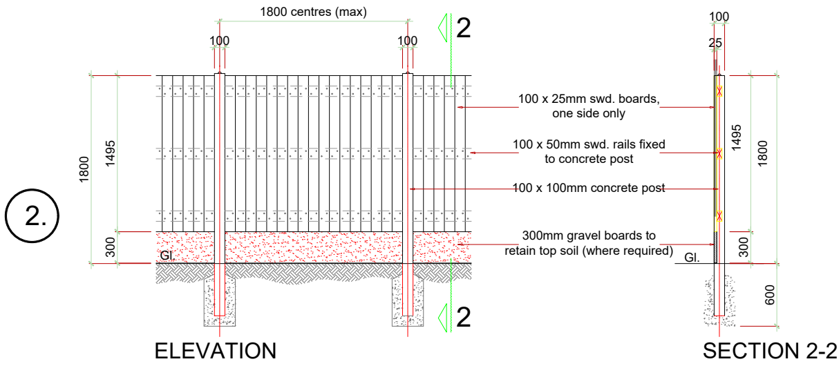
Typical Perimeter Fence detail 1.8m high Scale 1:50 @ A1 Fence - constructed in pretreated softwood with weathered rails bolted to concrete. Posts - set in concrete 600mm deep with concrete gravel boards where minor changes in levels occur and fixed to retaining wall where necessary.
