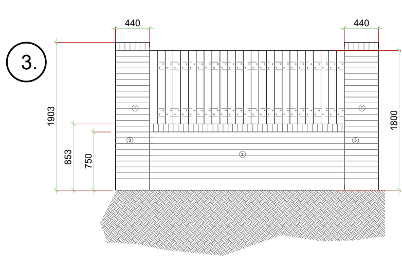
Feature wall detail 1.8m high Scale 1:50 @ A1 1. Brick on edge capping 2. 215 mm brick dwarf wall 3. 440 mm brick piers 4. Foundation to Structural Eng Design 5. Close board timber infill panel
