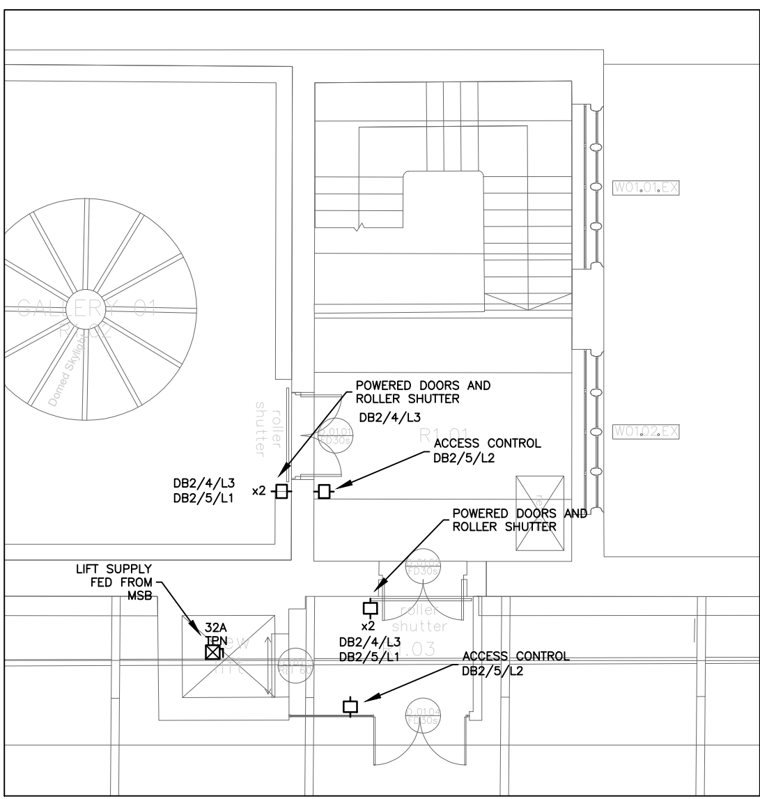
FIRST FLOOR SMALL POWER
