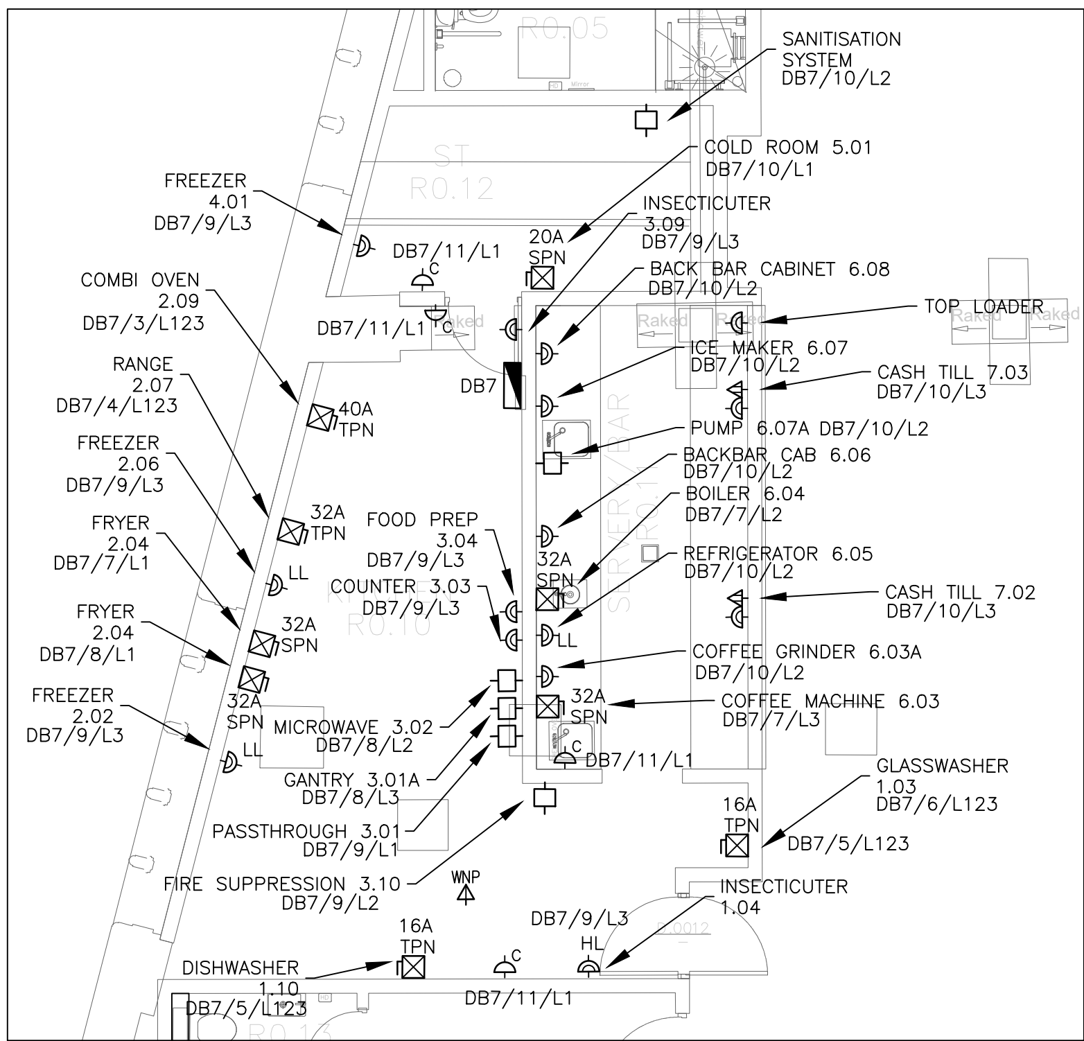
KITCHEN SMALL POWER
