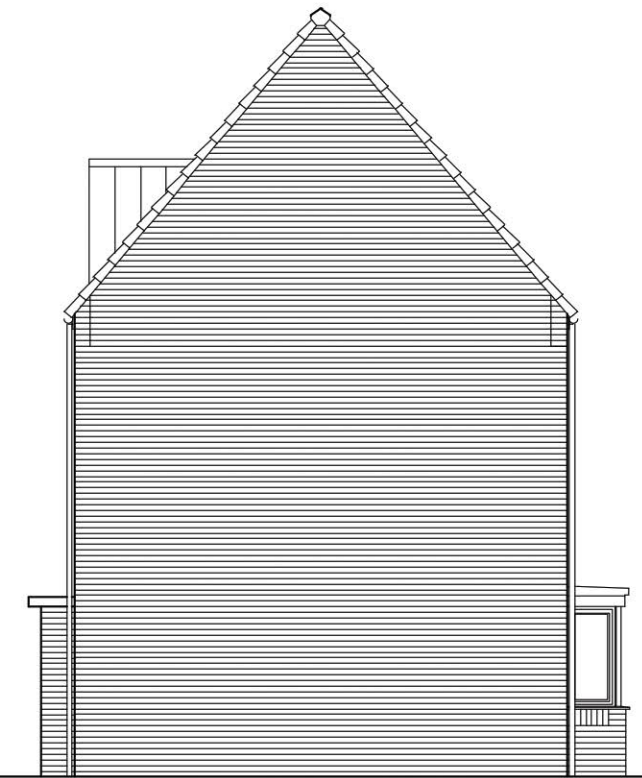
Side Elevation
