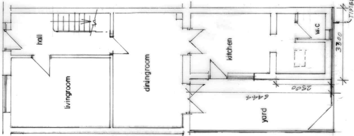
GROUND FLOOR PLAN (AFTER)
