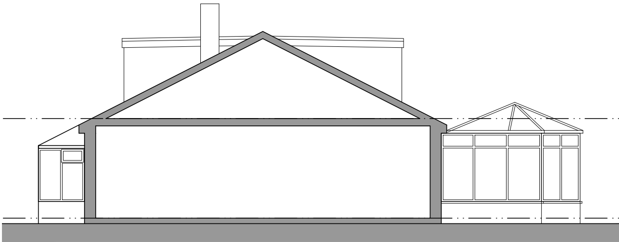
West Facing Side Elevational Section
