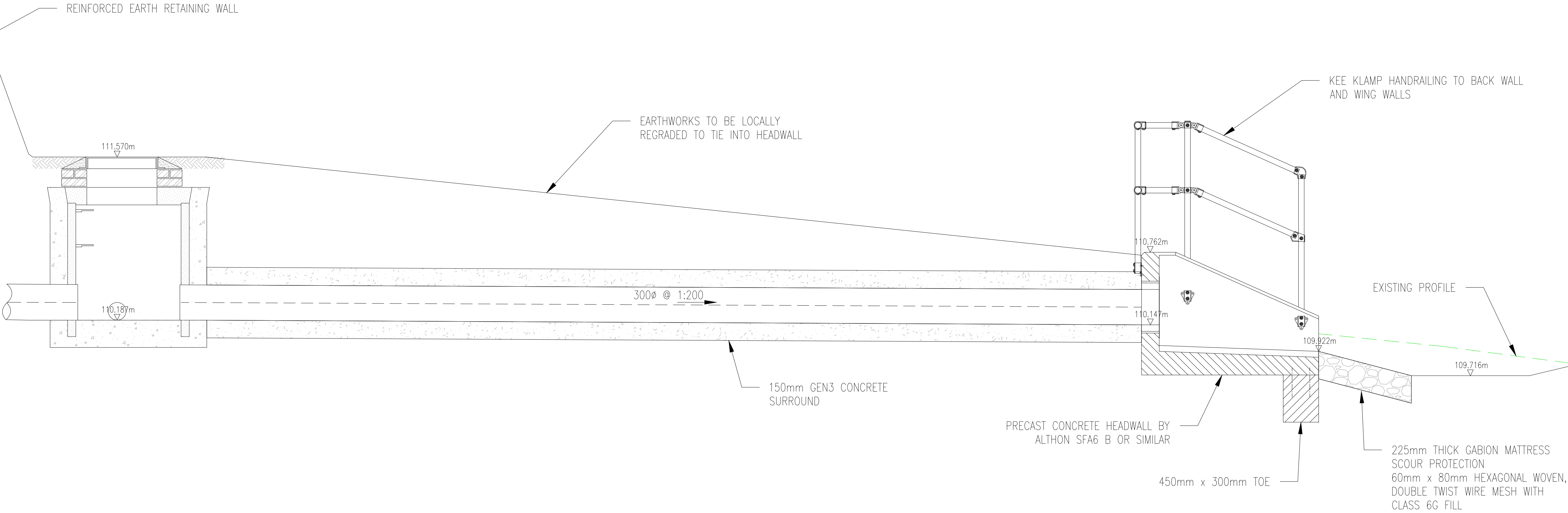
SURFACE WATER OUTFALL SECTION SCALE 1:20
