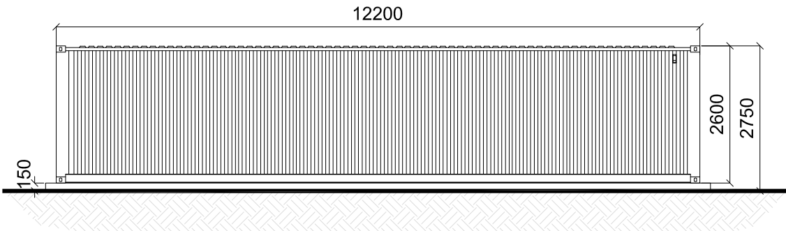
FRONT ELEVATION
