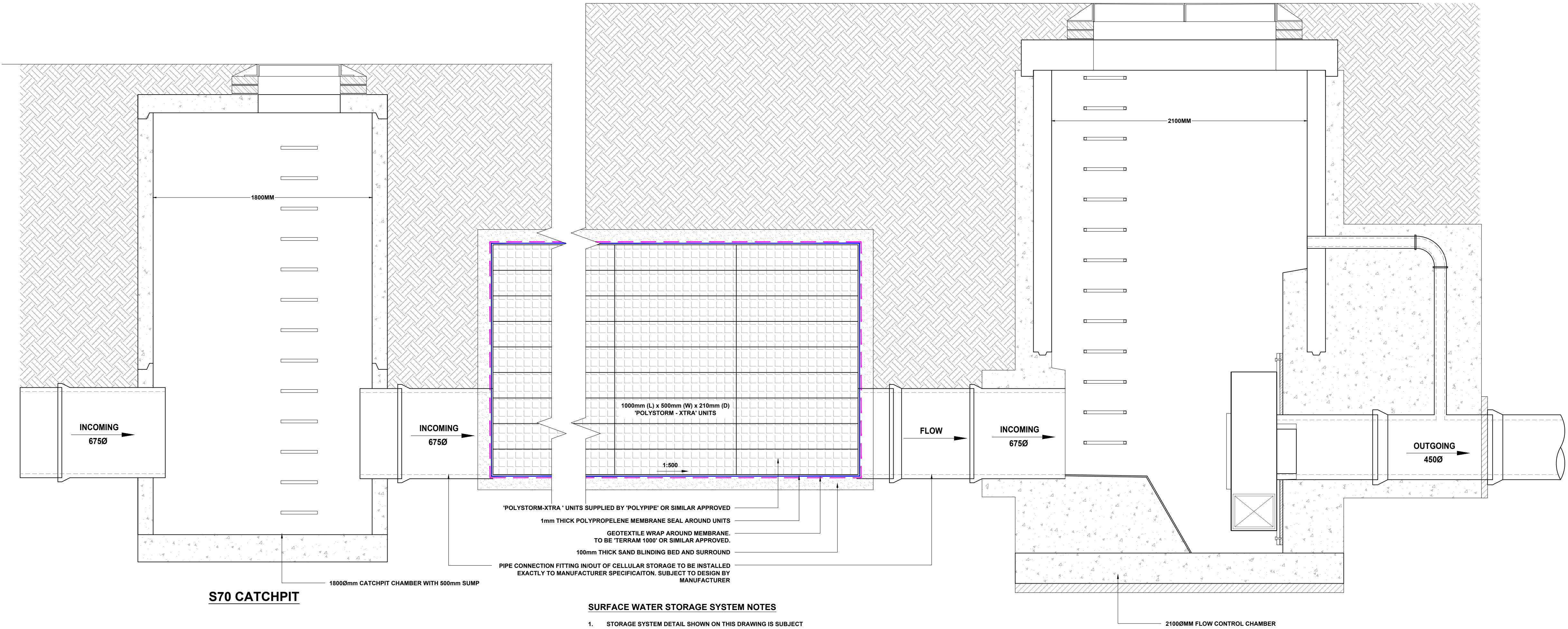
ONLINE 'POLYSTORM - XTRA - PSM3' (OR SIMILAR APPROVED) CELLULAR STORAGE TANK & CATCHPIT CHAMBER - TYPICAL CONSTRUCTION DETAIL
