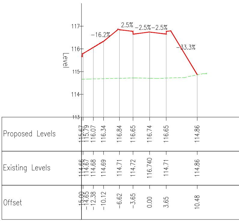
Chainage 120.000
