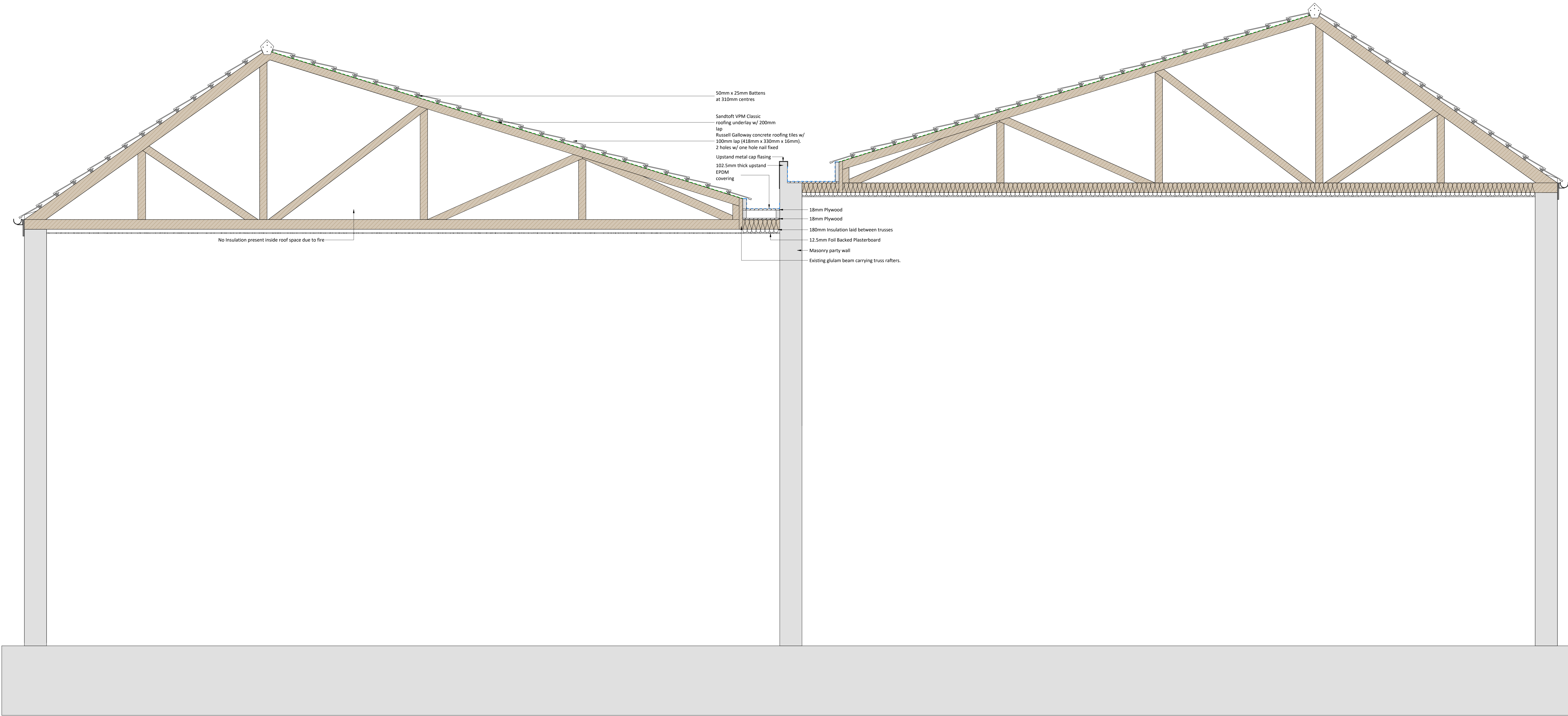
Roof Valley Gutter Detail - Existing 1 : 20
