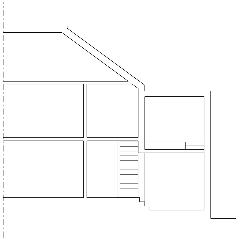
EXISTING SECTION A-A
