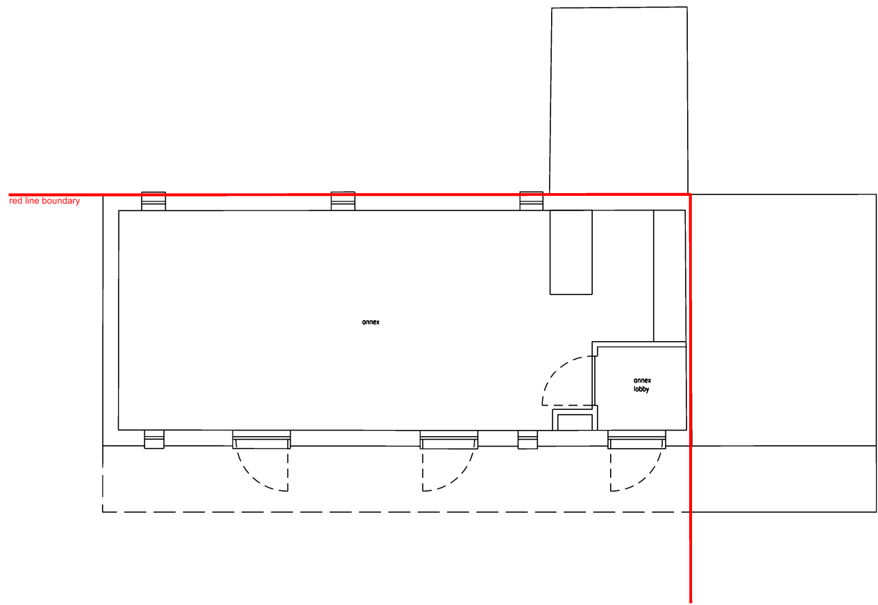
FLOOR PLAN
