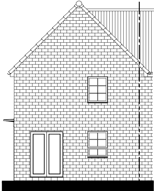
REAR ELEVATION
