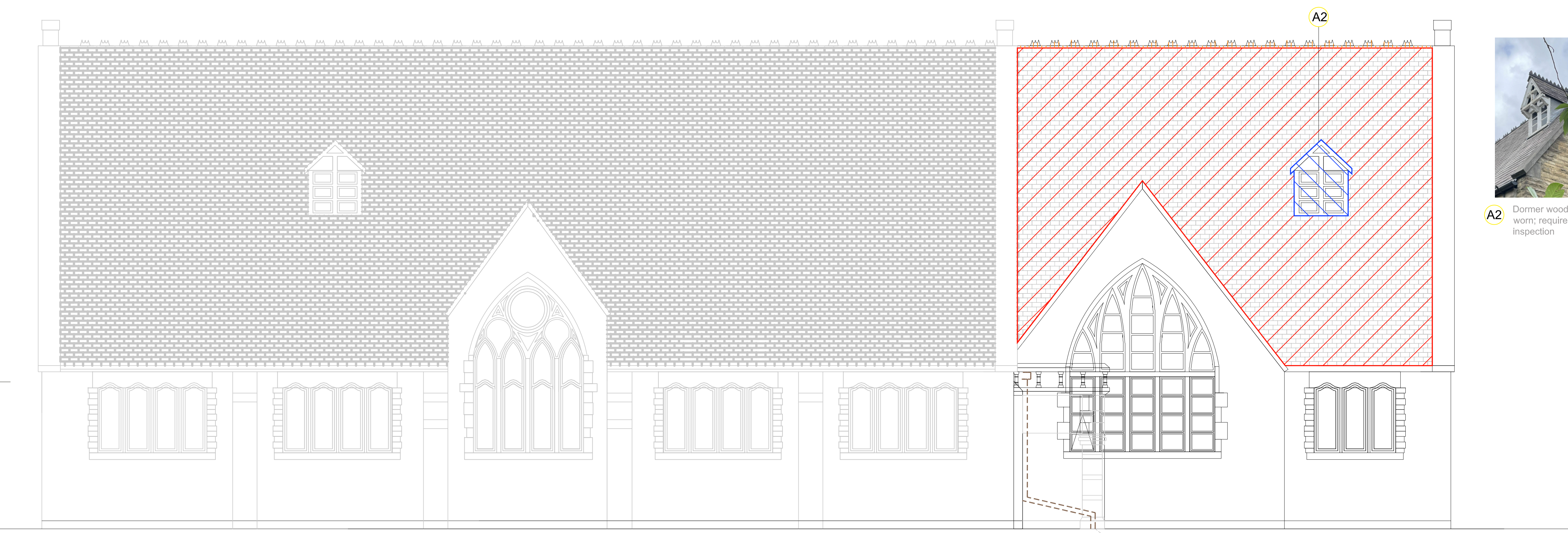
Elevation CC
