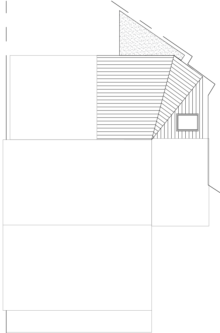
Roof Plan
