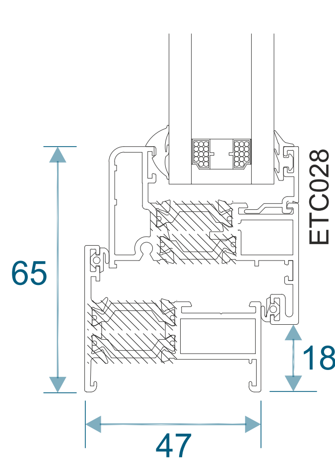
Opening Vents With ETC010 Outer Frame
