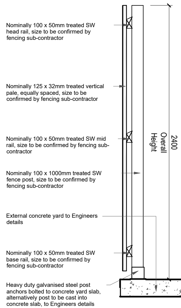
Bin Store Detail Section Scale @ 1:20
