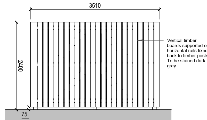
Rear Elevation Scale @ 1:50
