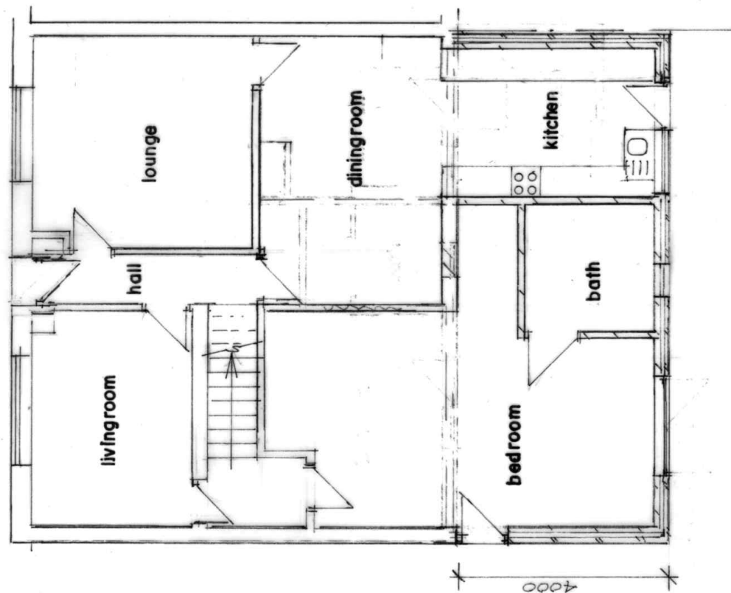
GROUND FLOOR PLAN (PROPOSED)
