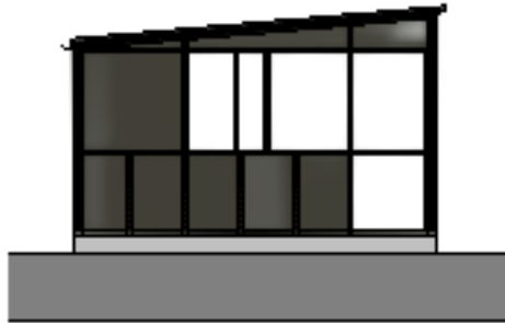
Proposed North East Elevation
